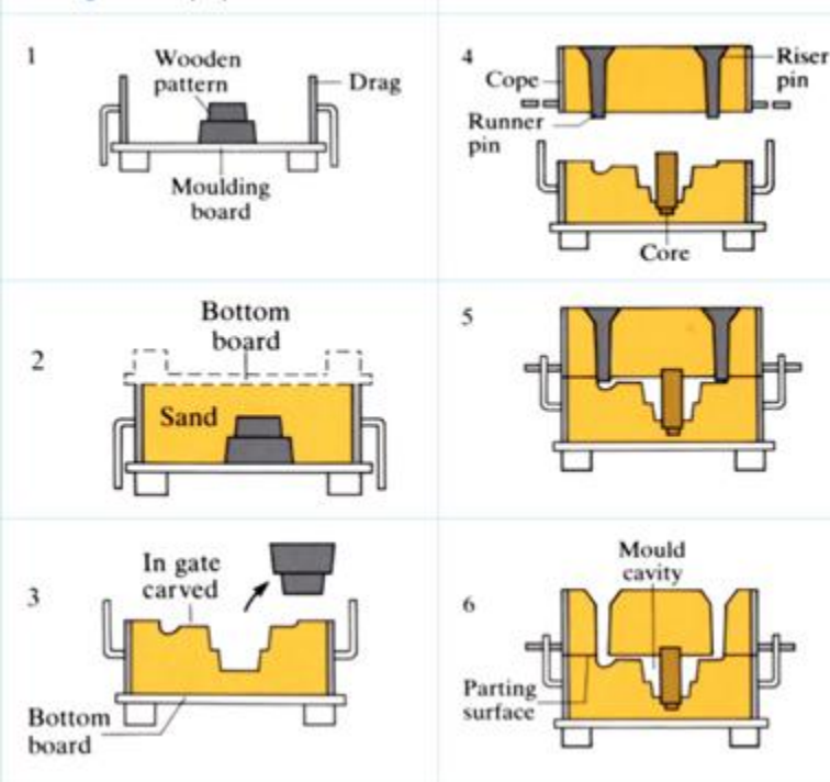
Moulding with a simple pattern
